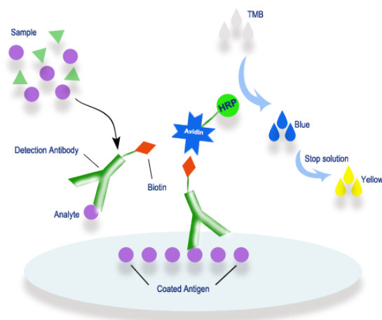
(2) Competitive-ELISA
