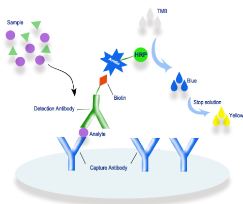
(1) Sandwich-ELISA
