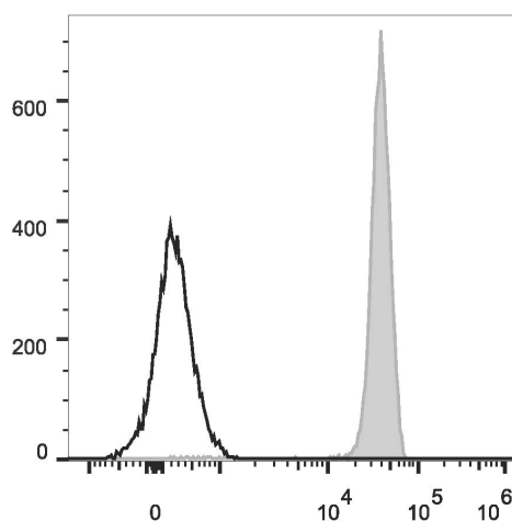
Human peripheral blood lymphocytes are stained with PerCP Anti-Human CD45 Antibody (filled gray histogram). Unstained lymphocytes (empty black histogram) are used as control.
