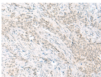
Immunohistochemistry of paraffin-embedded Human ovarian cancer tissue using HABP4 Polyclonal Antibody at dilution of 1:60(×200)
