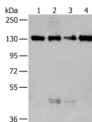
Western blot analysis of 293T and 231 cell lysates using MORC2 Polyclonal Antibody at dilution of 1:250
