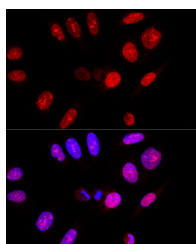
Confocal immunofluorescence analysis of U-2 OS cells using Ataxin 3 Polyclonal Antibody at dilution of 1:100. Blue: DAPI for nuclear staining.
